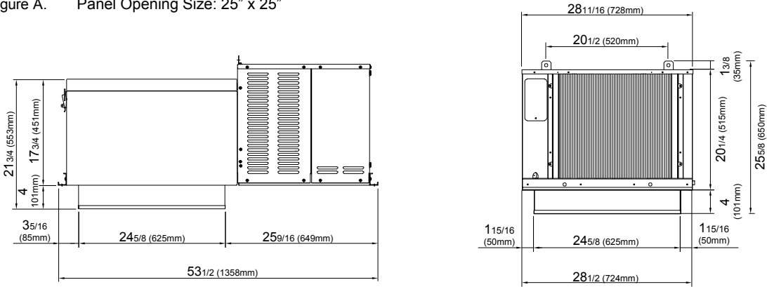
Figure A. Panel Opening Size: 25" x 25"
