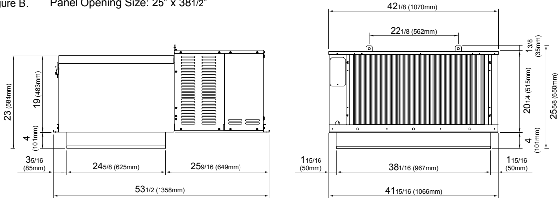
Figure B. Panel Opening Size: 25" x 38 1/2"
